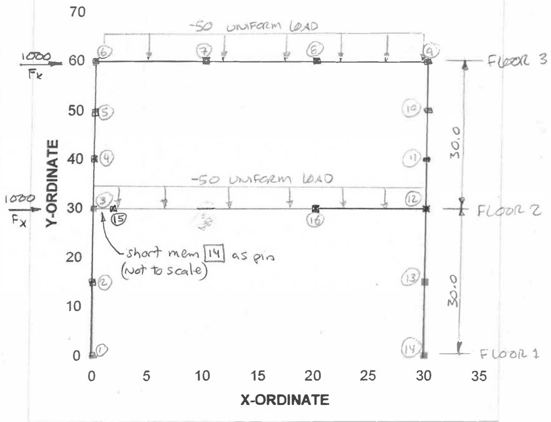
FIGURE 5: BUILDING EXAMPLE NODE & MEMBER PLOT, with LOADINGS
