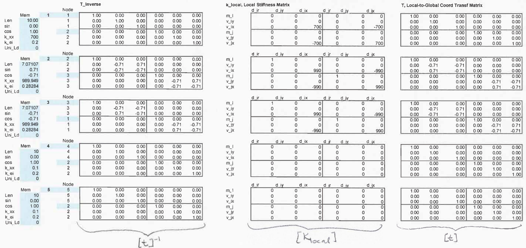
FIGURE 6: LOCAL STIFFNESS + COORDINATE TRANSFORMATION MATRICES FOR EXAMPLE 2 MODEL
